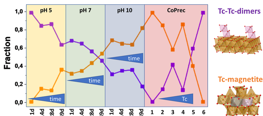
Figure 4. Species distribution of \text{Tc}^{\text{IV}}\text{--Tc}^{\text{IV}} -dimers sorbed on magnetite (purple) and \text{Tc}^{\text{IV}} -substituted magnetite (orange) for Tc sorption on magnetite at different pH (5.0, 7.0 and 10.0) and contact times (7, 14, 28, and 49 days) and in Tc coprecipitates in magnetite (CoPrec, Table S1) with increasing Tc loading; numbers correspond to number in Table S1.
