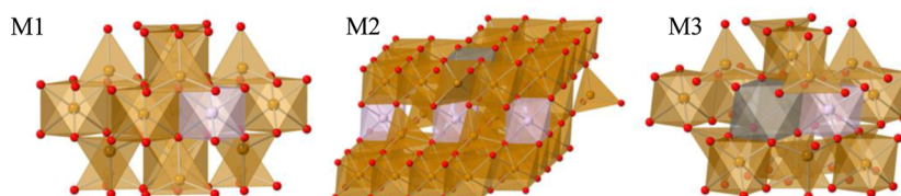
Figure 3. Tc IV -substituted magnetite corresponding to mechanisms mentioned above (M1, M2, M3). The structures were refined by DFT. Brown is Fe, pink is Tc, and gray is a vacancy.
